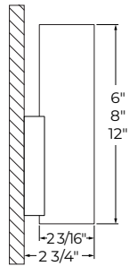
Direct mount 2
