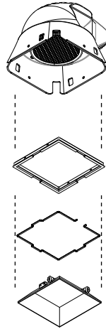
Trimless Millwork
