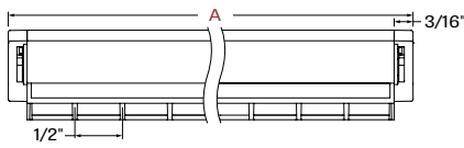
PIVWW - Pivot Wall Wash - Side view
