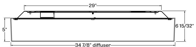
POROS + 5H - pop round surface-wall with 5" optics
