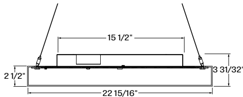
POSQPD + 2H - Pop Square Pendant with 2.5" optic
