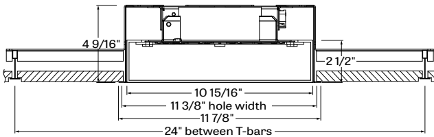
POSQR- TG15 - tegular 15/16"
