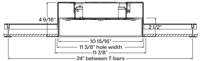
POSQR- ST - screw slot t-bar
