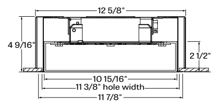
POSQR- DF - drywall kit
