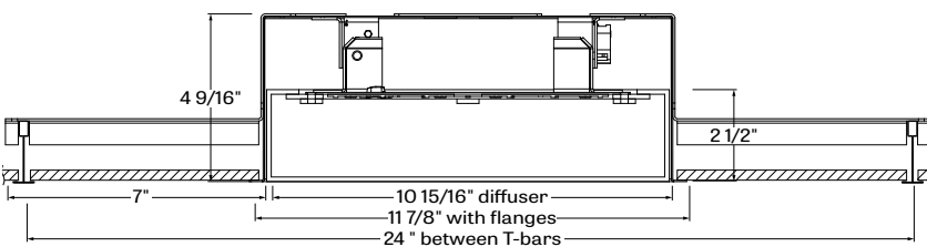
POSQR + FH - pop square recessed with flush lens
