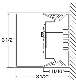
QUAWW - quad wide wall - DRM
