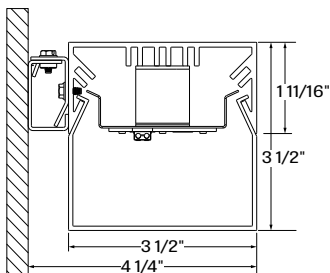
QUAWW - quad wide wall - DMB
