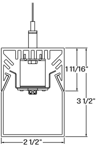
QUANP - air craft cable - narrow
