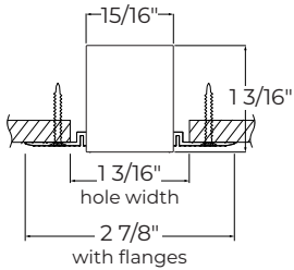
DMF - Drywall mud flange
