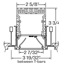
TG9 - Tegular 9/16"
