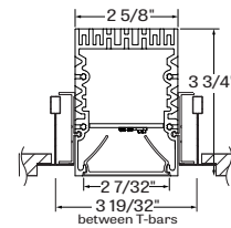
TG15 - Tegular 15/16"
