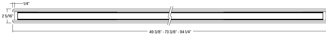
Bottom view
