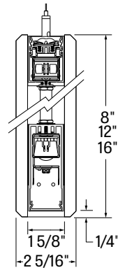
Section View
