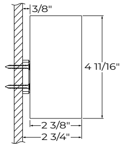
MMB - Mullion mounting bracket
