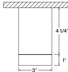
1.0" Drop Lens 1
