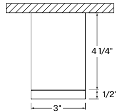
0.5" Drop Lens 1
