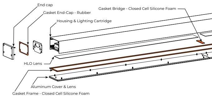
Lens and enclosure are sealed with inner and outer silicone gaskets
